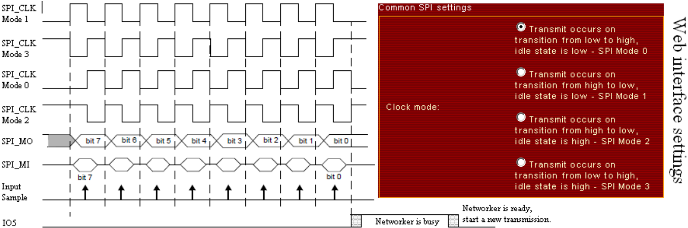
Fig. 2: Waveforms
