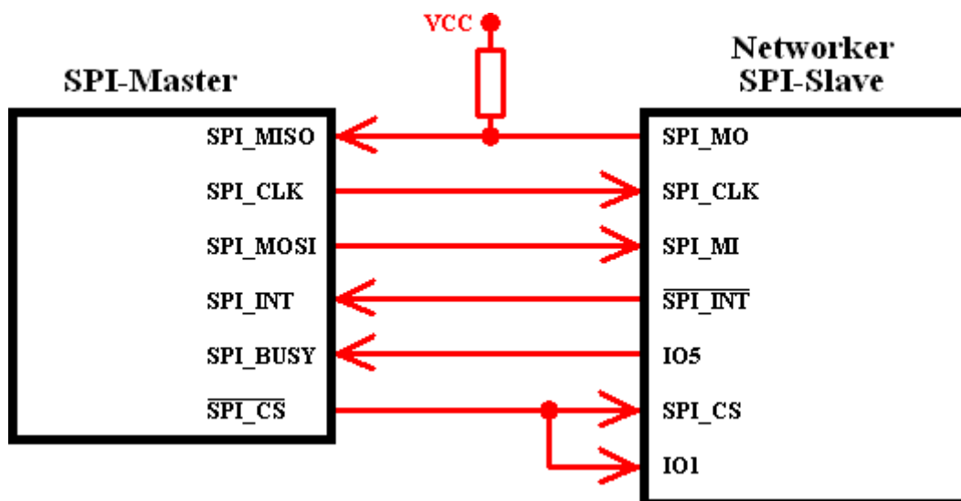
Fig. 1: Connection example
